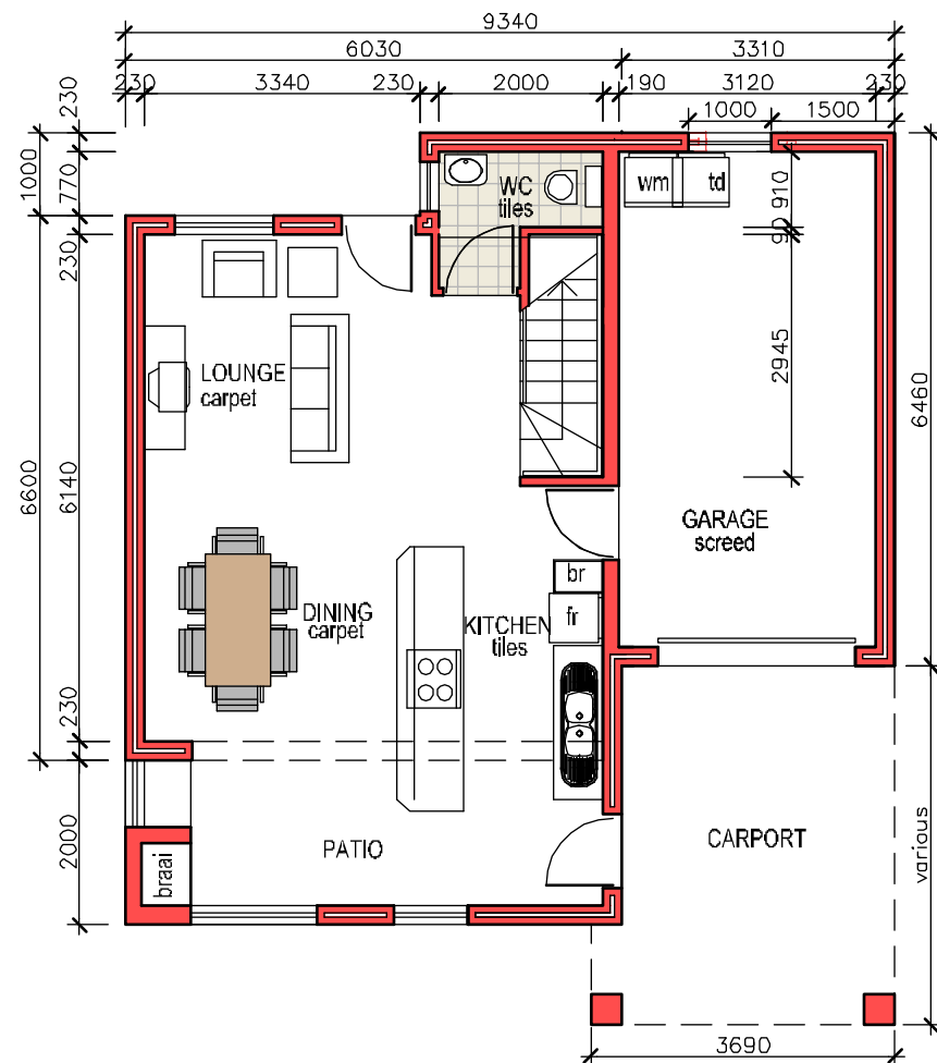
GROUND FLOOR - TYPE E
