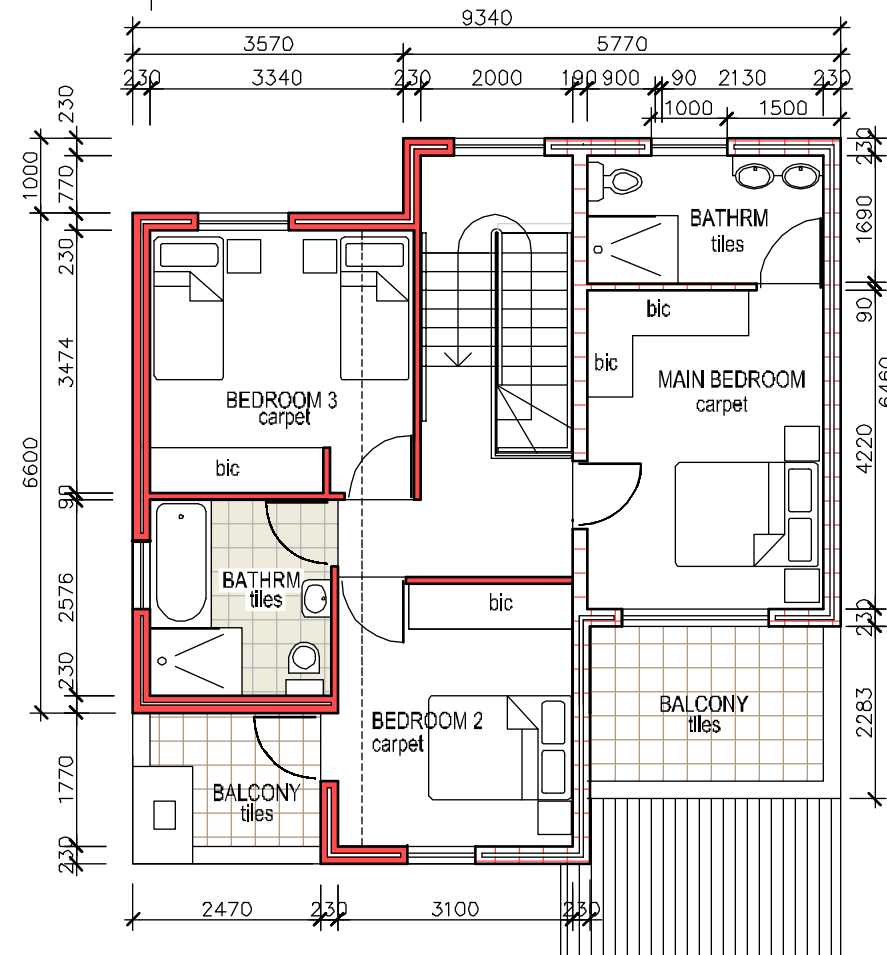
FIRST FLOOR - TYPE E
