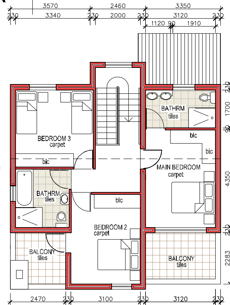
FIRST FLOOR - TYPE A
