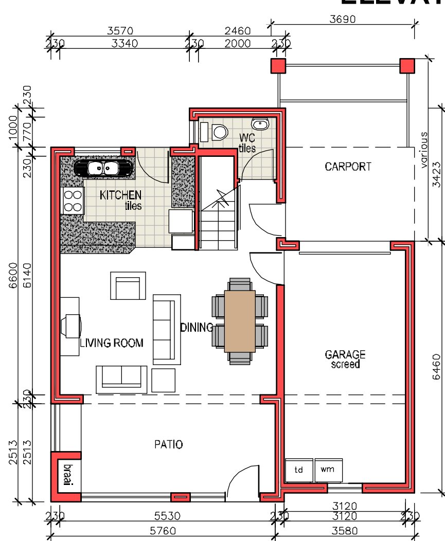
GROUND FLOOR - TYPE A
