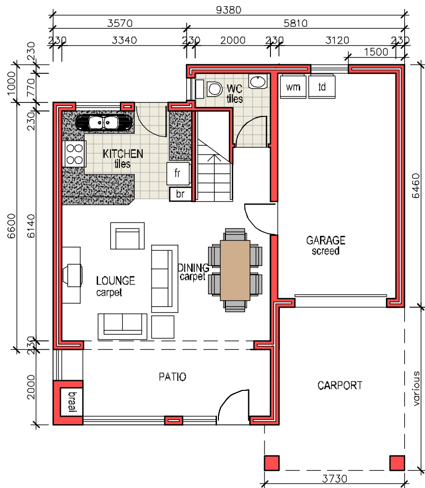
GROUND FLOOR - TYPE B
