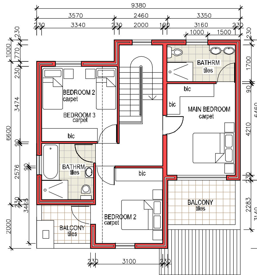
FIRST FLOOR - TYPE B
