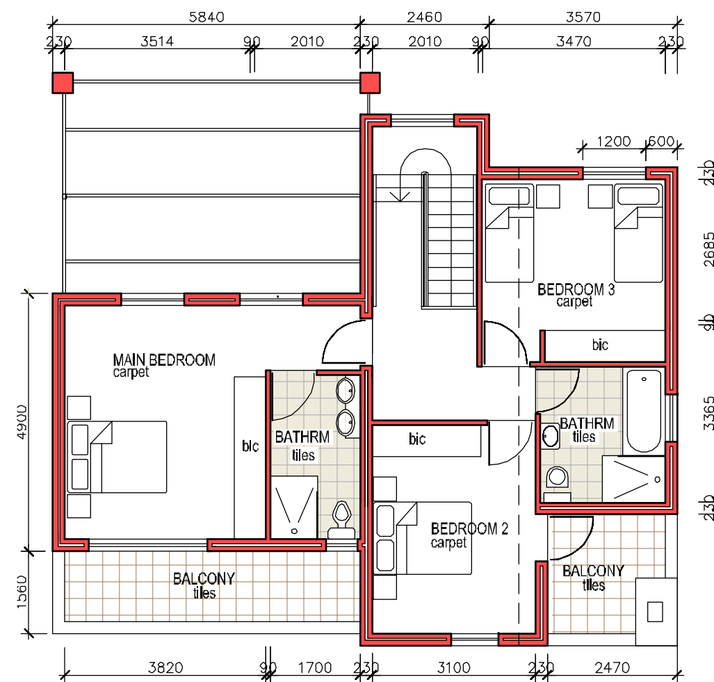
FIRST FLOOR - TYPE C
