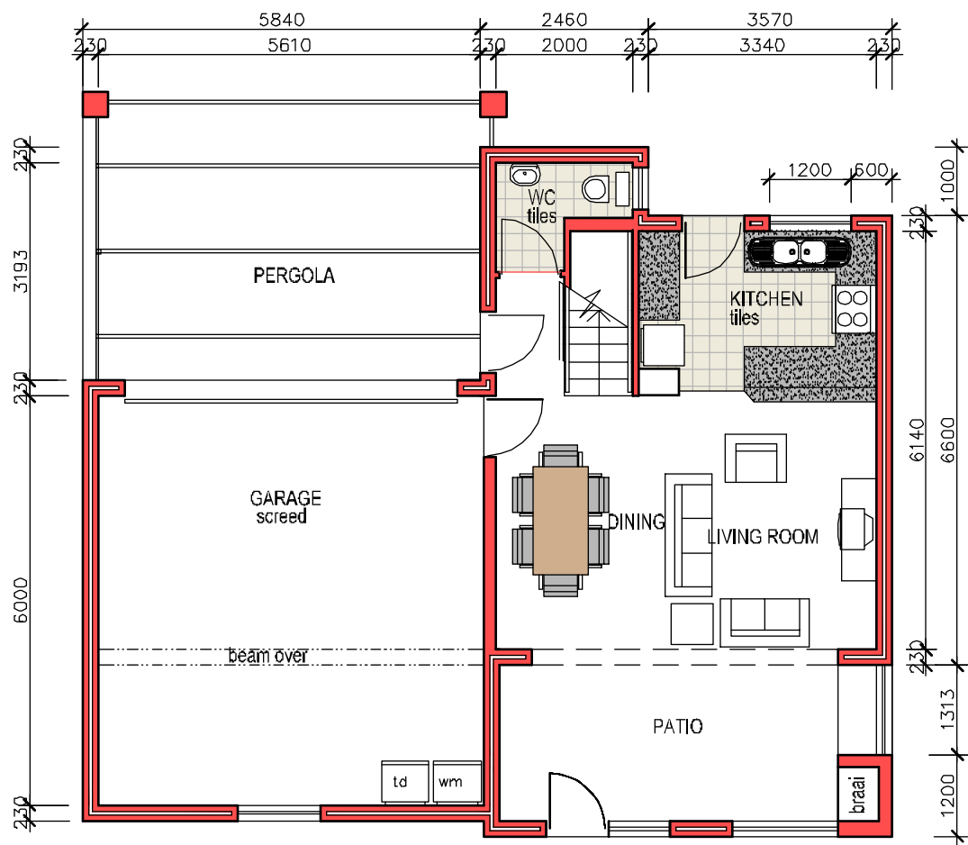
GROUND FLOOR - TYPE C
