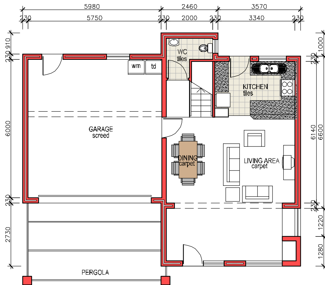
GROUND FLOOR - TYPE D
