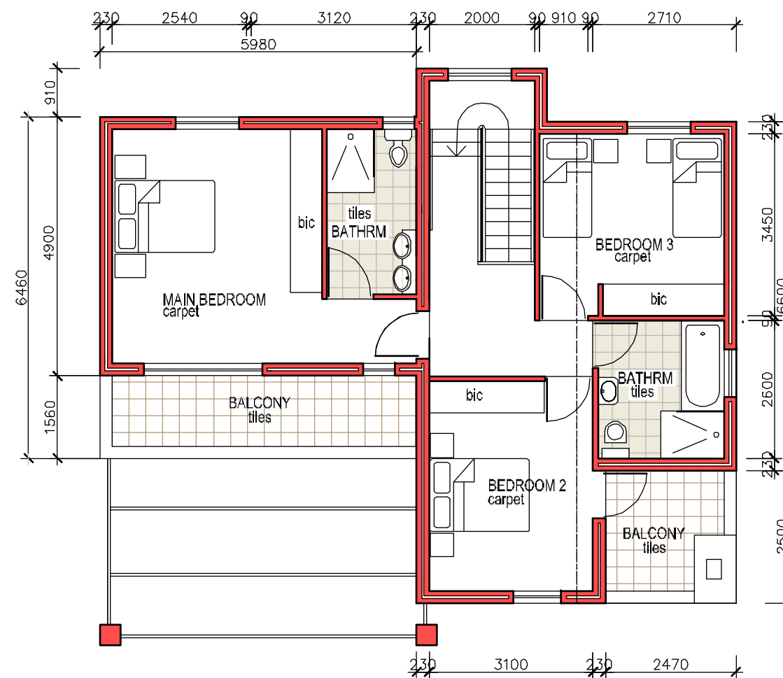
FIRST FLOOR - TYPE D
